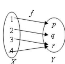
Surjective
