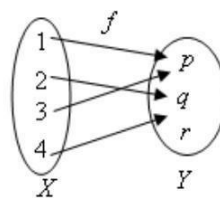
Not Surjective
