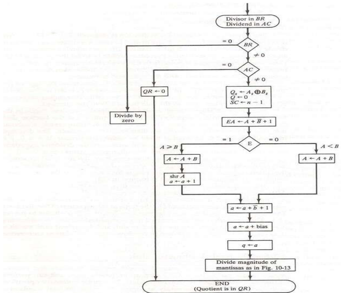
Figure 10-17 Division of floating-point numbers.
