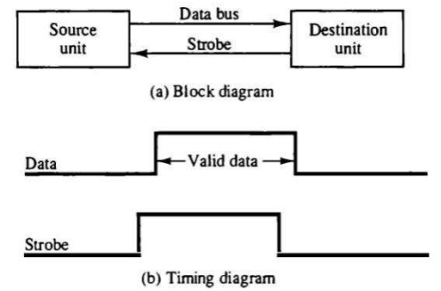
Destination-initiated strobe for data transfer.
