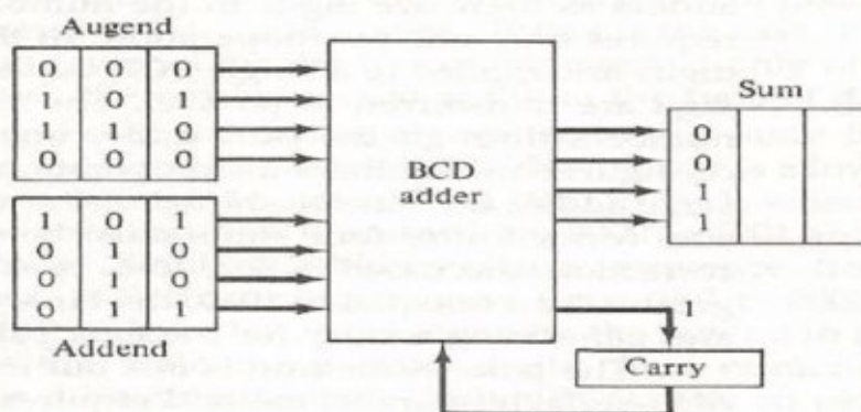
(b) Digit-serial, bit-parallel decimal addition
