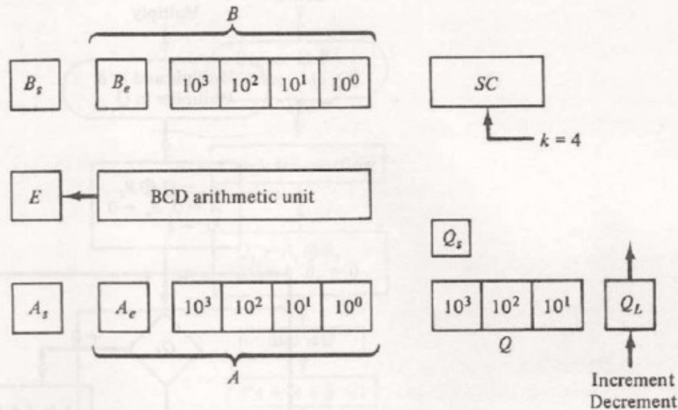
Figure 10-21 Registers for decimal arithmetic multiplication and division.
