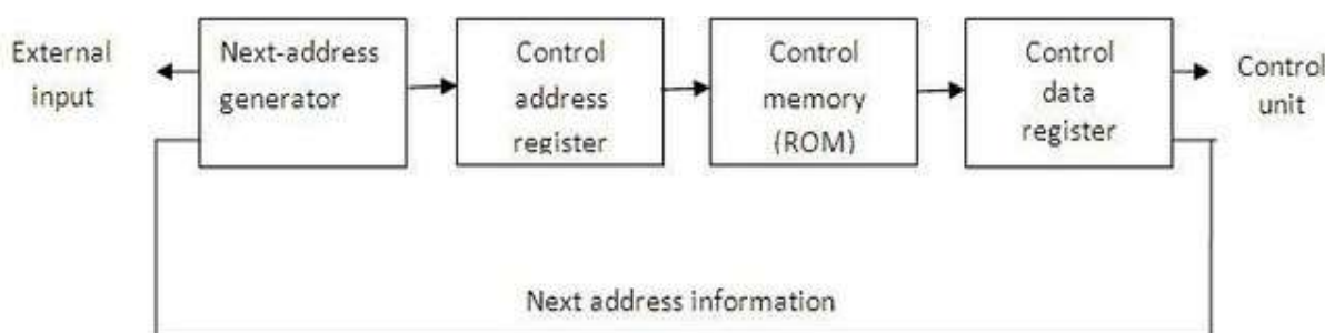
figure 4.1: Micro-programmed control organization
