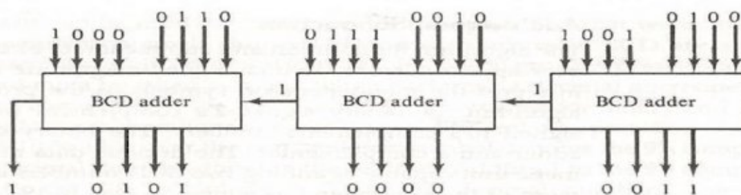
(a) Parallel decimal addition: 624 + 879 = 1503
