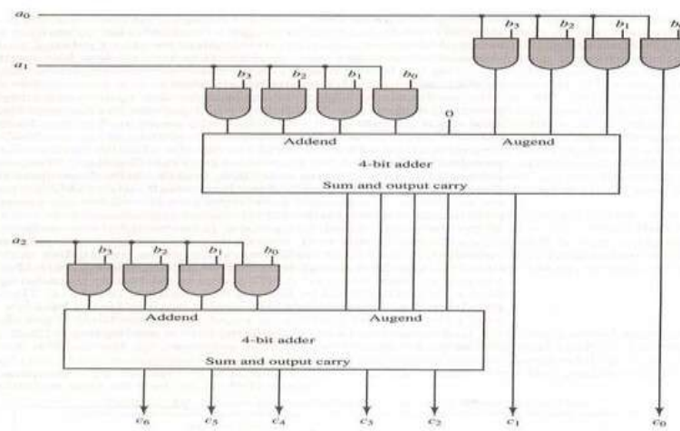
Figure 10-10 4-bit by 3-bit array multiplier.
