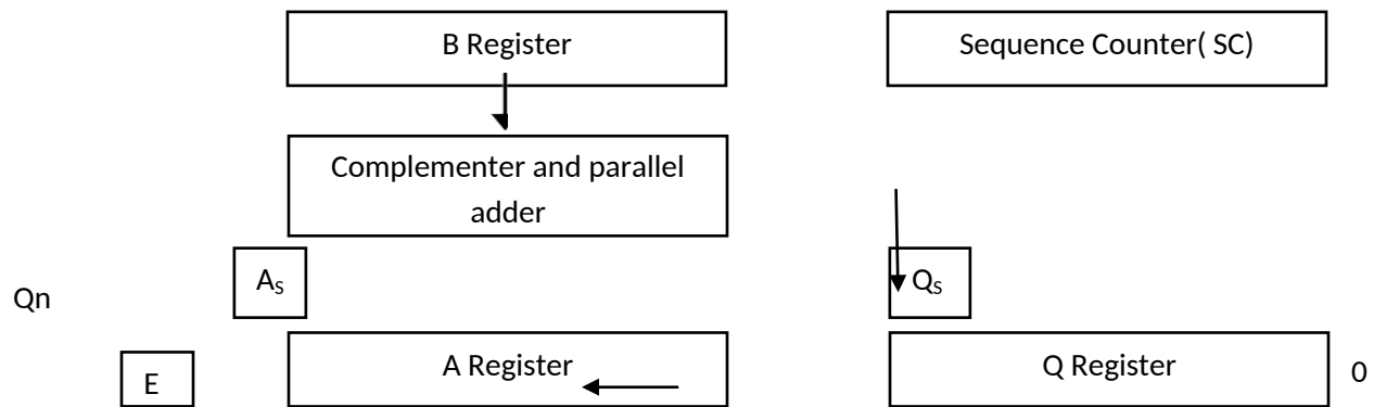
Hardware for implementing division of fixed point signed- Magnitude Numbers
