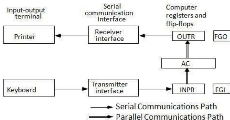
Figure 2.12: Input-output configuration
