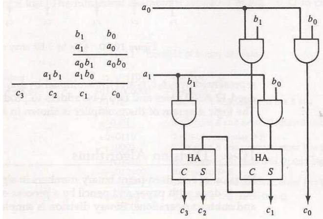
Figure 10-9 2-bit by 2-bit array multiplier.
