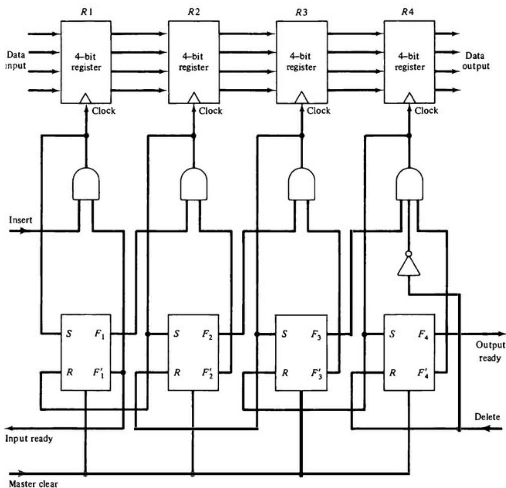
Figure 11-9 Circuit diagram of 4 \times 4 FIFO buffer.
