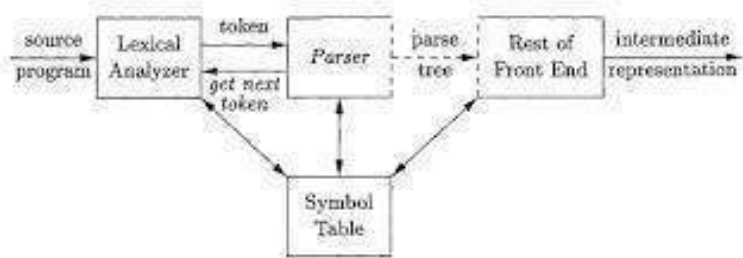
Figure 4.1: Position of parser in compiler model
