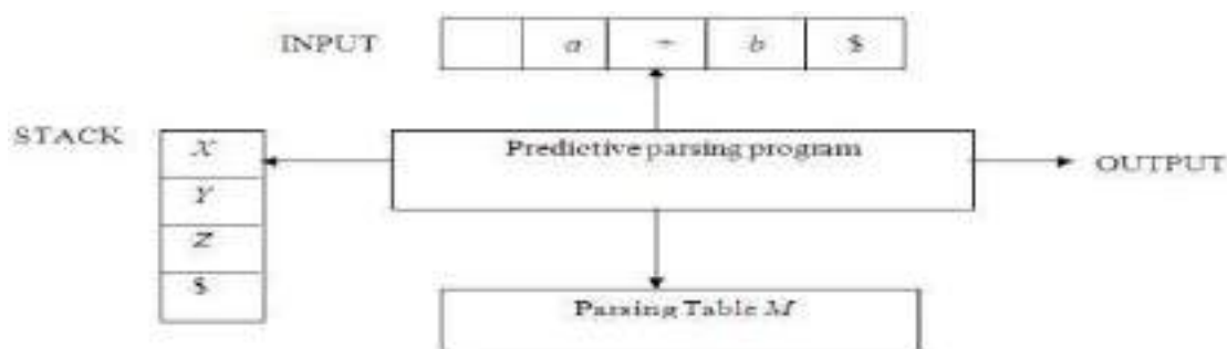
Fig. 2.4 Model of a nonrecursive predictive parser
